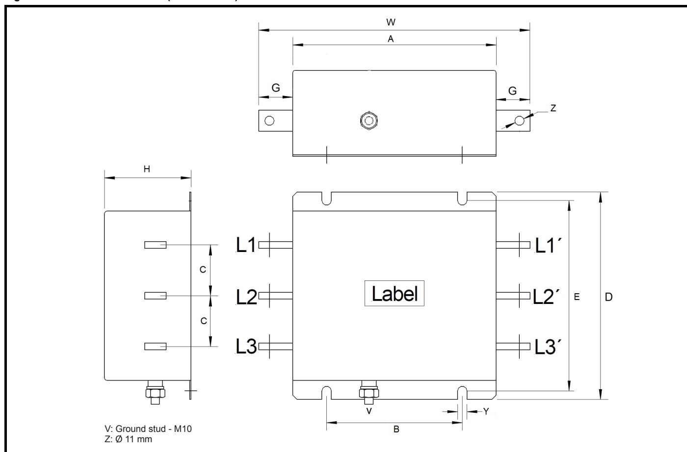
Figure 5-42 External EMC filter (size 9 and 10)
