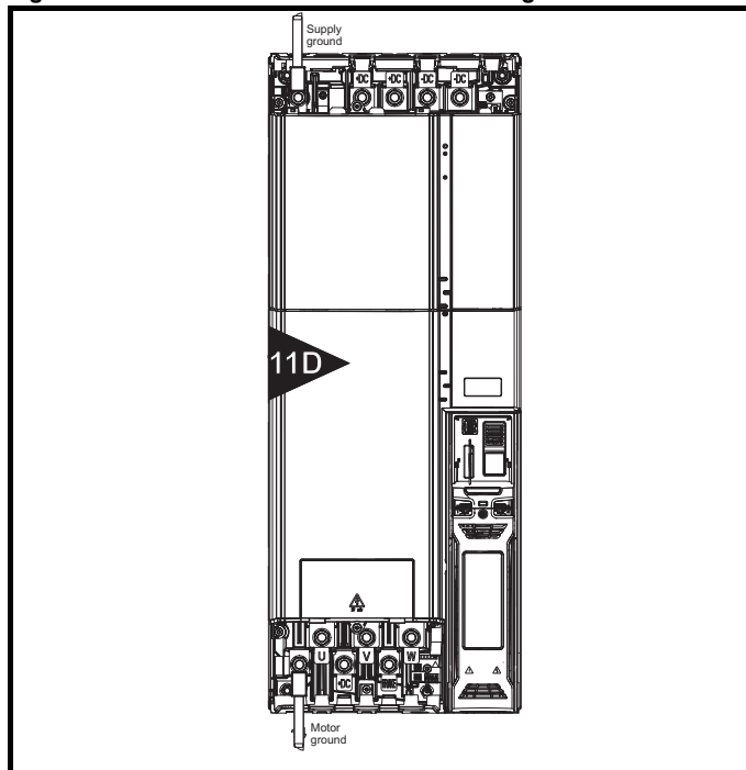
Figure 6-13 Unidrive M/Unidrive HS size 10 rectifier ground connections
