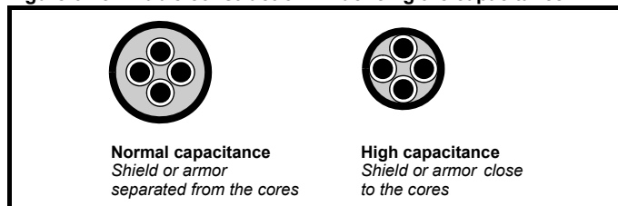
Figure 6-18 Cable construction influencing the capacitance
