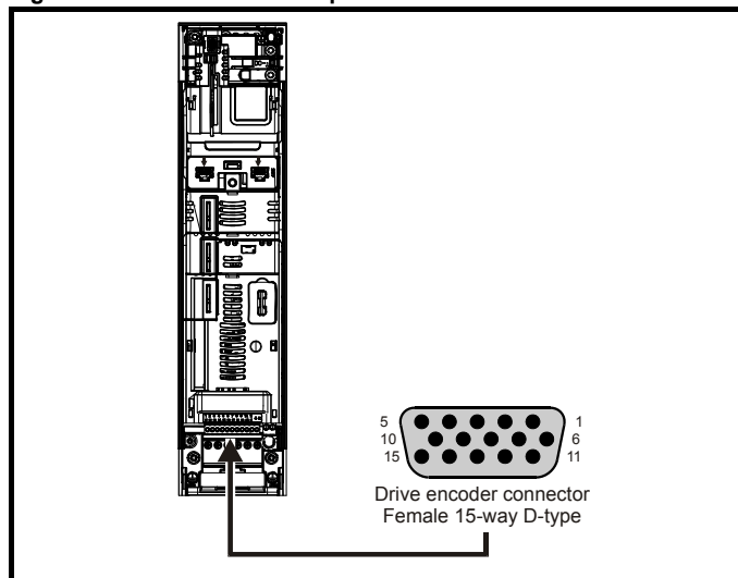
Figure 6-42 Location of the position feedback
