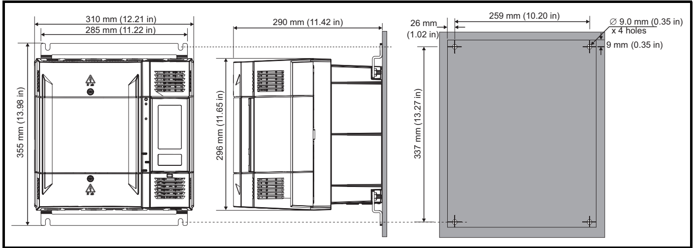
Figure 5-18 Surface mounting the Unidrive M / Unidrive HS size 11 rectifier
