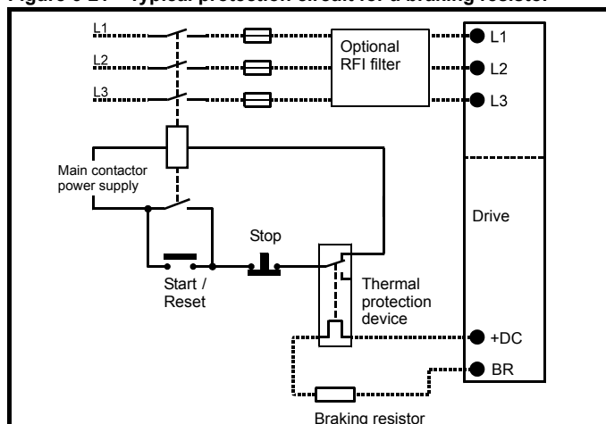
Figure 6-21 Typical protection circuit for a braking resistor
