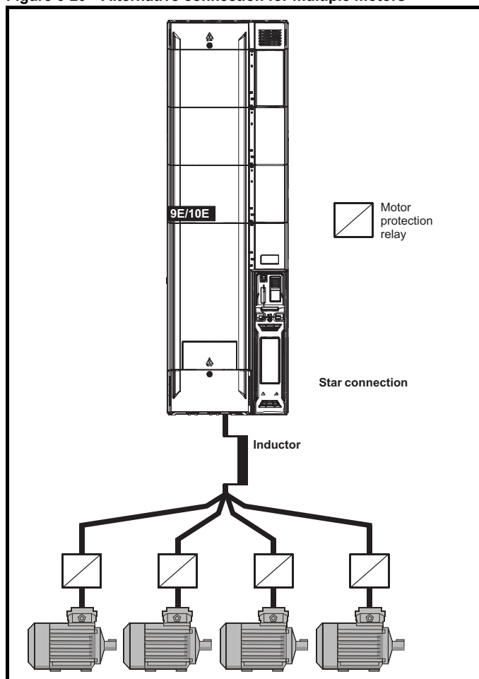
Figure 6-20 Alternative connection for multiple motors
