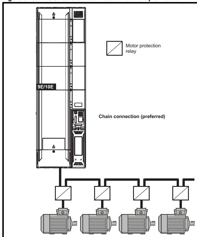
Figure 6-20 Alternative connection for multiple motors
