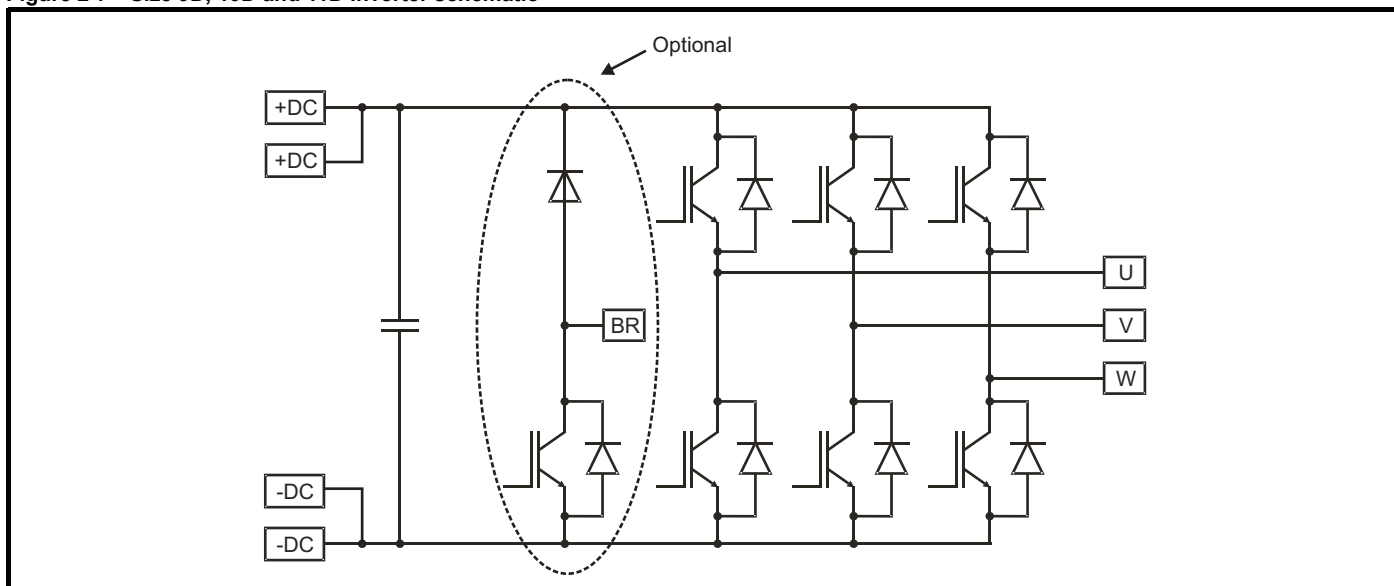
Figure 2-7 Size 9D, 10D and 11D inverter schematic
