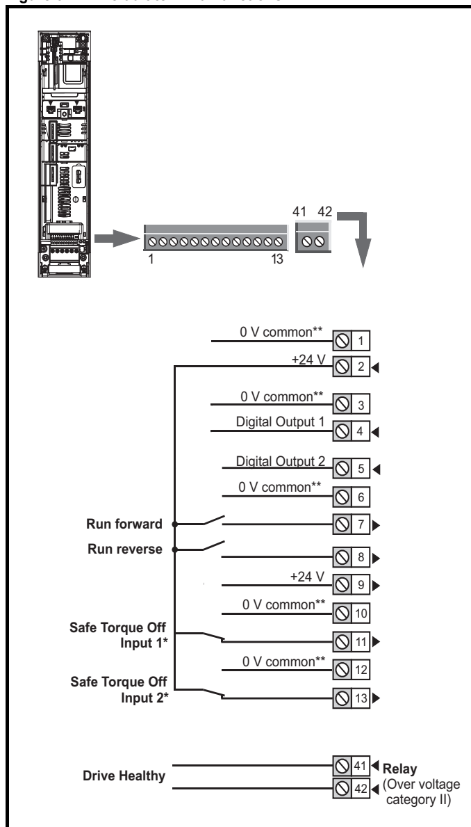
Figure 6-41 Default terminal functions
