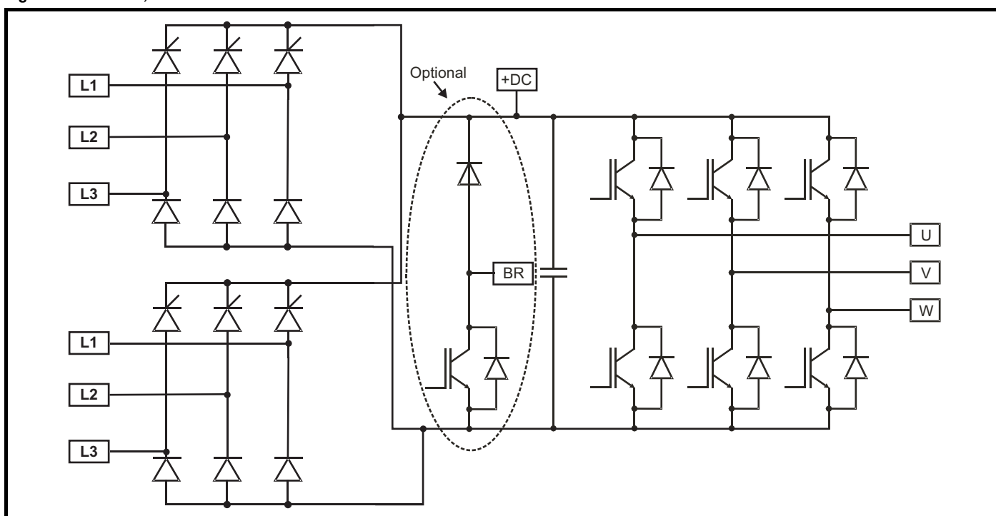
Figure 2-8 Size 9T, 10T and 11T inverter schematic
