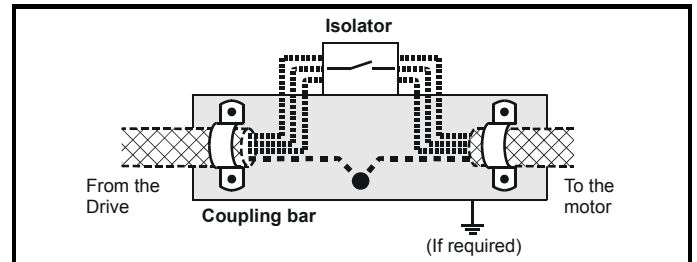
Figure 6-35 Connecting the motor cable to an isolator/disconnect switch
